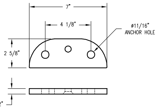
SURFACE MOUNT PLATE DETAIL
